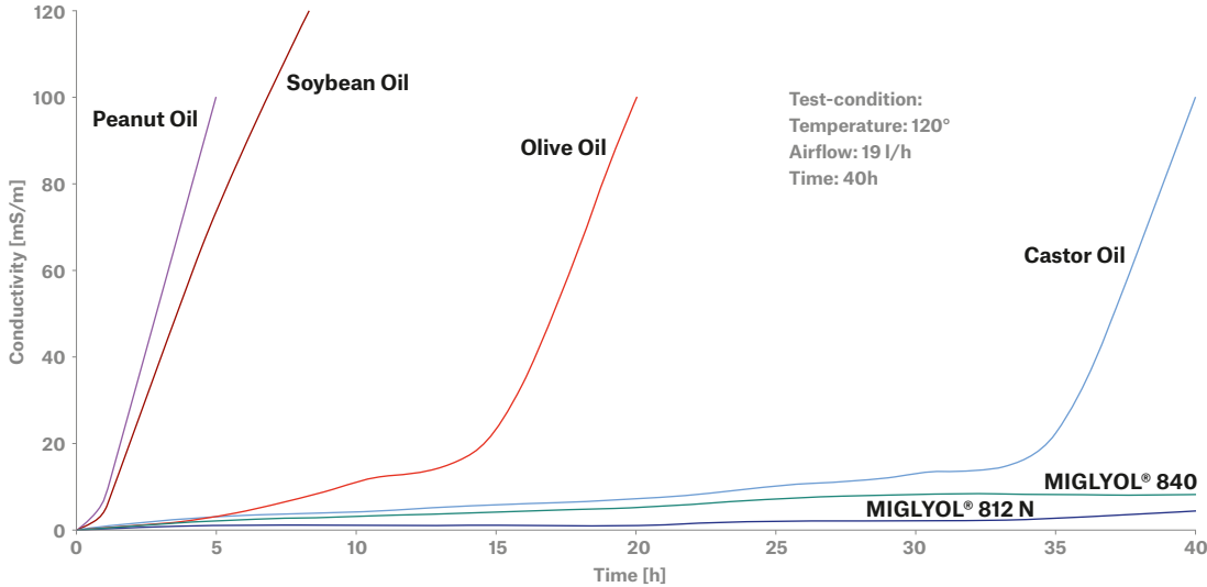
The conductivity increases exponential when the natural content of antioxidants in vegetable oil is consumed and the capacity to resist autoxidation is exhausted
